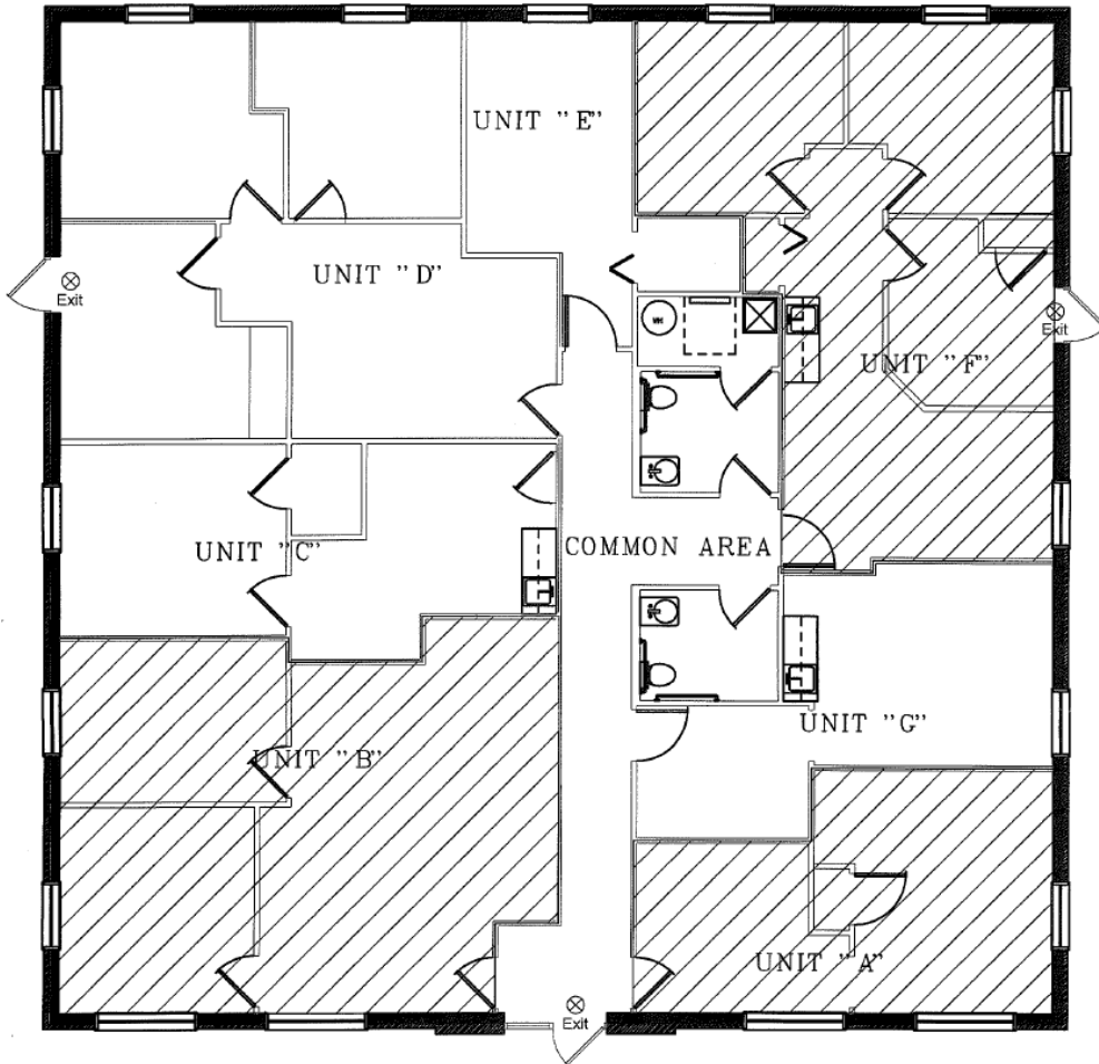
FLOOR PLAN
